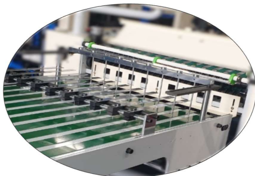
Auto Stacking & Conveying Unit
